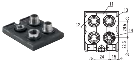
I/O cover (3M12 | 1 pin, 2 socket)
