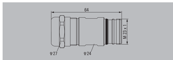
Figure 2: M23 coupling connector
