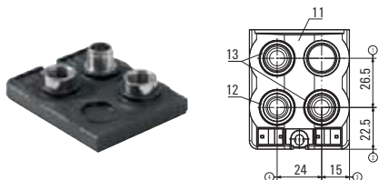
LP I/O cover (4M12 | 2 pin, 2 socket)
