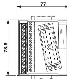
Чертеж UMK-EC56/25/EX-R
