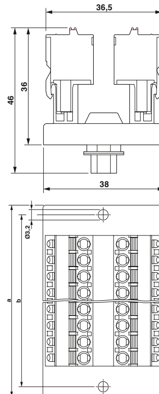
Чертеж DFLK-D...SUB...FKCT
