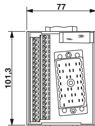
Чертеж UMK-EC90/32/EX-XUR
