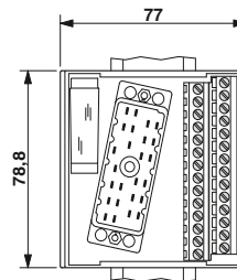
Чертеж UMK-EC56/25/EX-L
