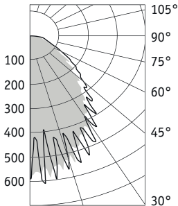
ALS.PRS UNI LED 600×600 4000 K
