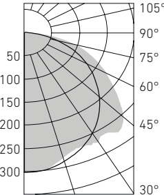
SLICK.OPL LED 50 5000K
