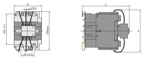
CJ19-115~170
