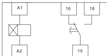
NJS5-M2
