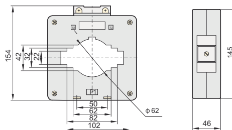
BH-0.66 100 I
