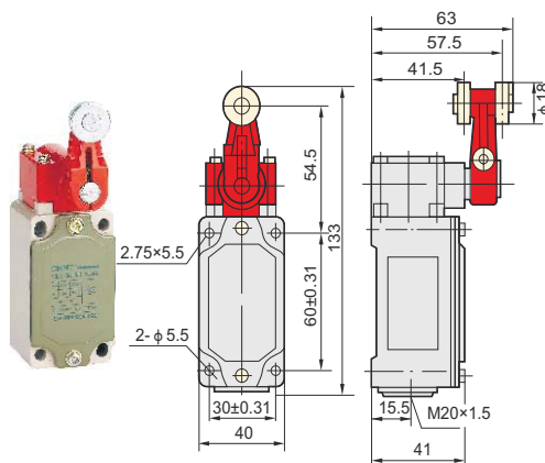
YBLX-K3/20S/B
