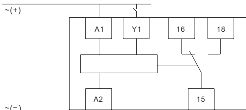
NJS5-M2
