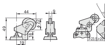
YBLX-P1/100/F YBLX-P1/120/F
